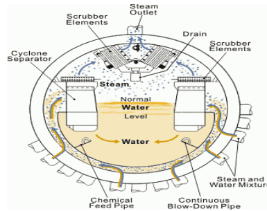
Gambar 5. Steam Drum
