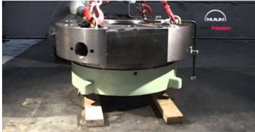
Gambar 1 Cylinder Head KM. Cakra Kembar Satu
