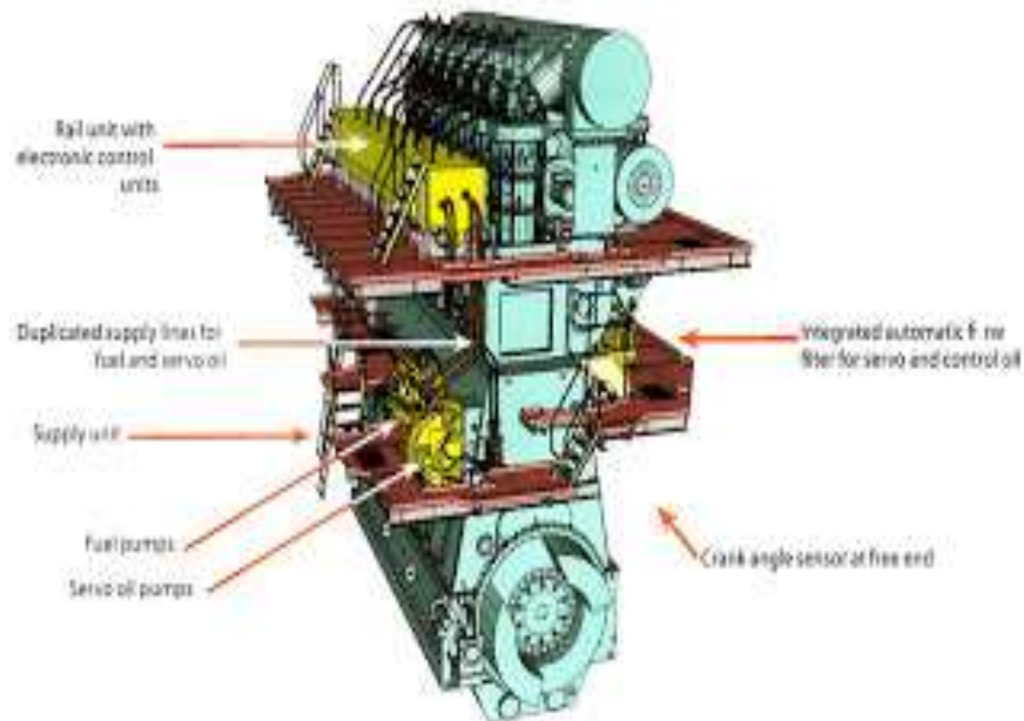
Gambar 10. Skema Safety Main Engine
