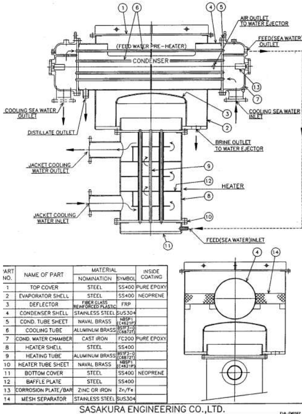
Gambar 1 Bagian masing-masing fresh water generator
